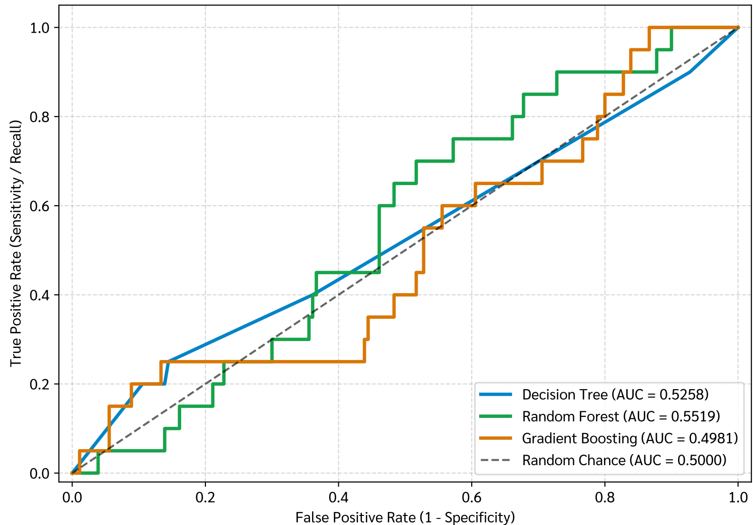
Receiver Operating Characteristic (ROC) Curves Comparison
